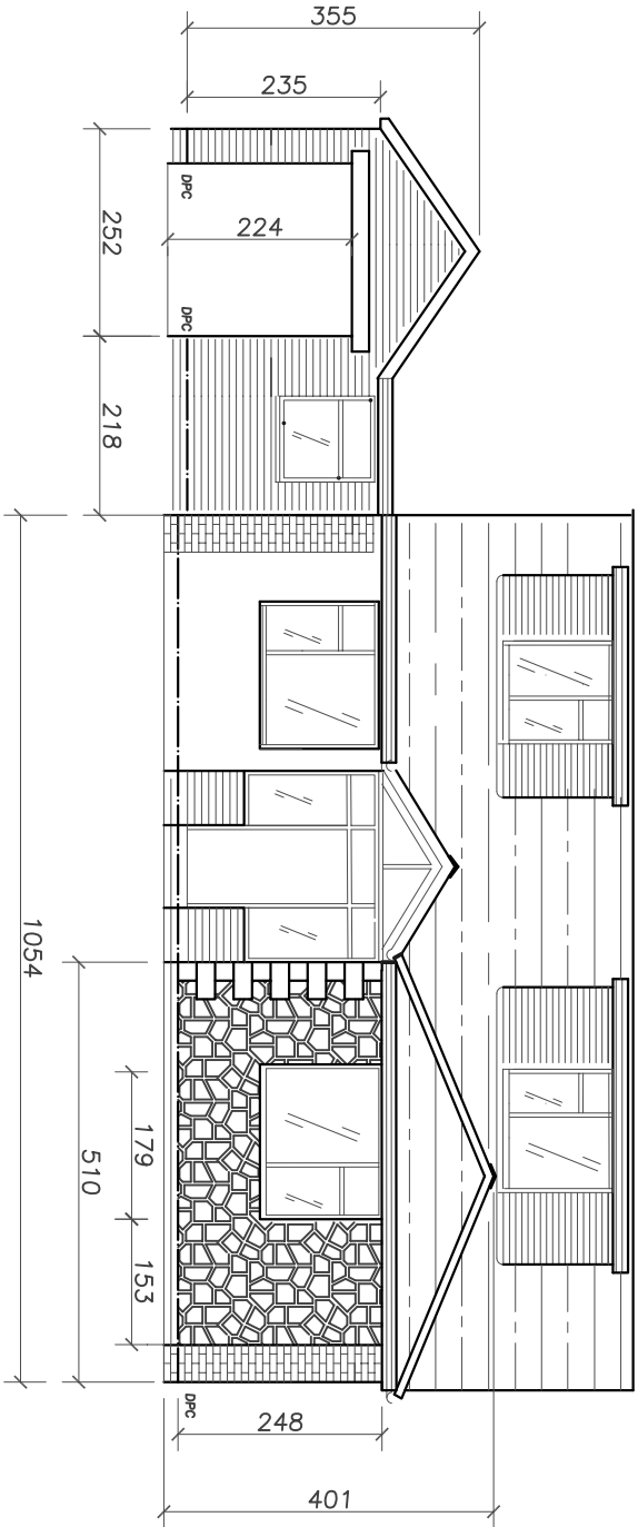
Front Elevation
