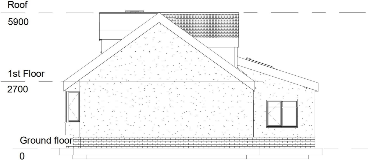
Proposed Side Elevation - RH (3)
