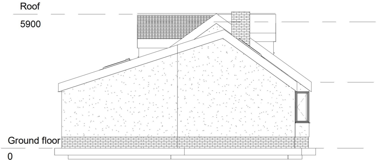
Proposed Side Elevation - LH (4)
