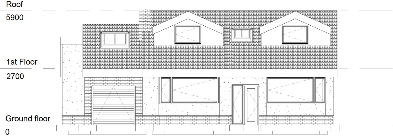
Proposed Front Elevation (1)
