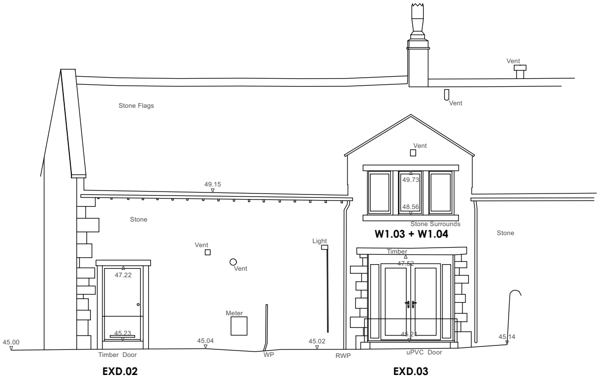
2 EXISTING EAST ELEVATION 1:100
