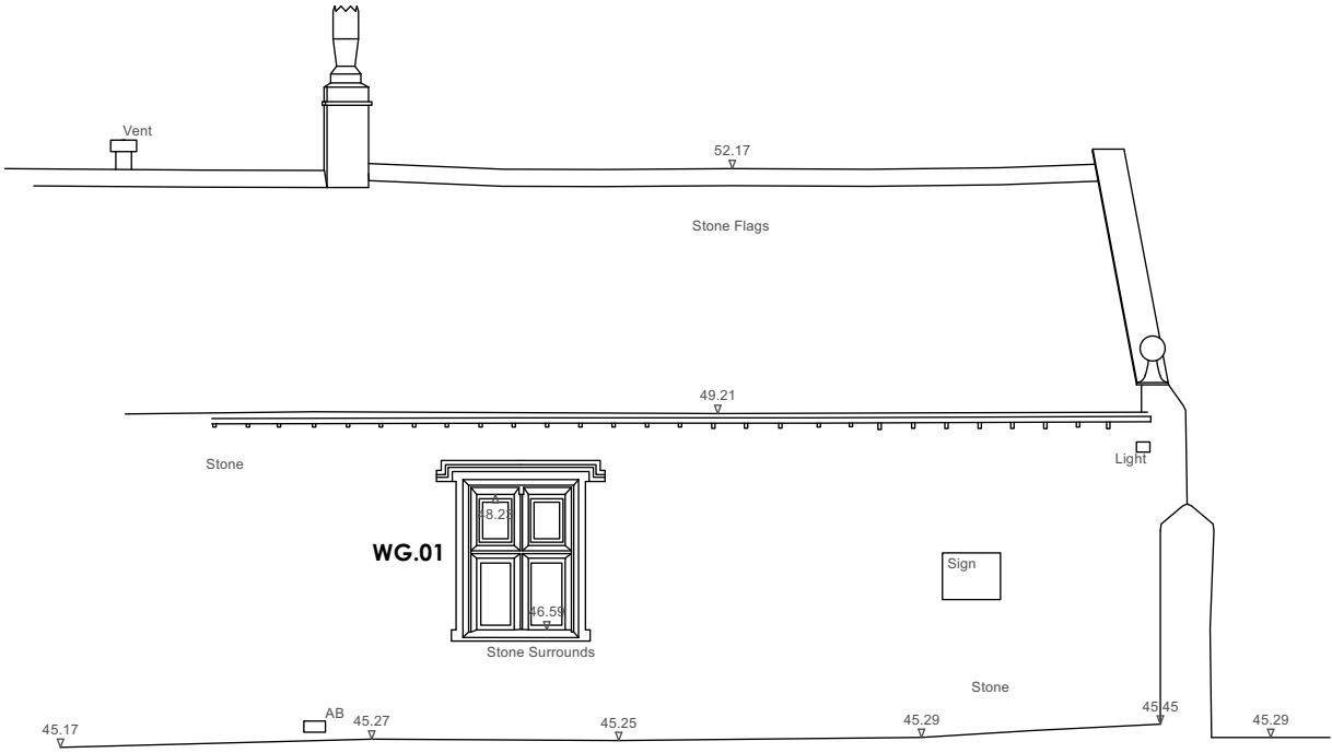
1 EXISTING WEST ELEVATION 1:100
