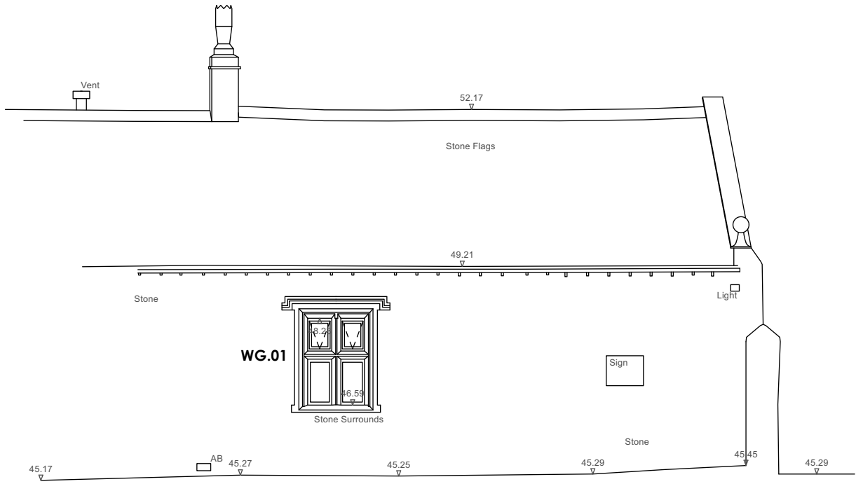
1 PROPOSED WEST ELEVATION 1:100
