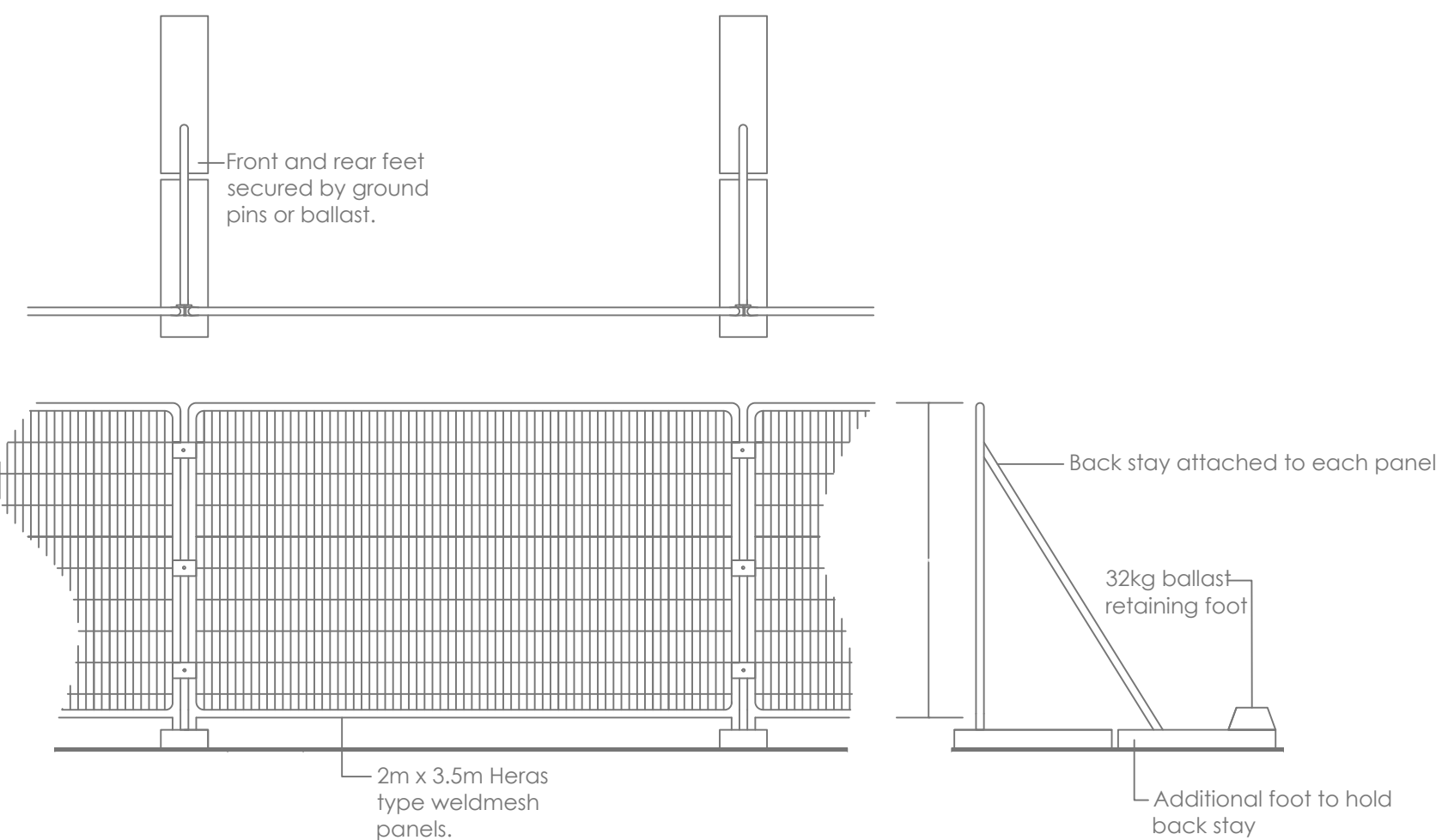
Back-stay support
