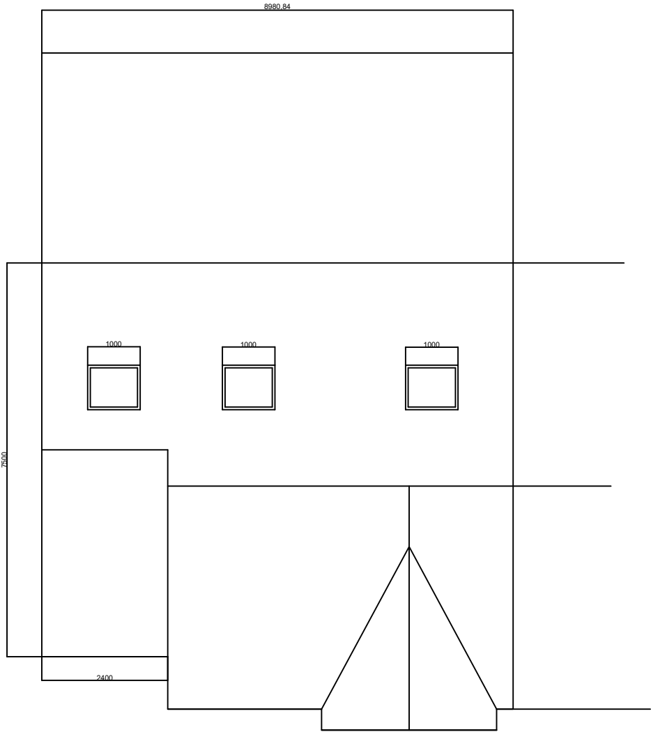
ROOF PLAN
