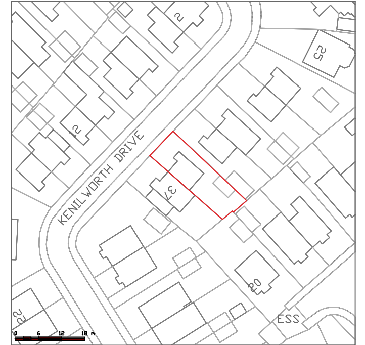
Block Plan
