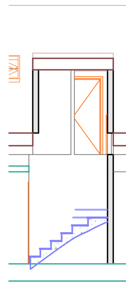
Building Section
