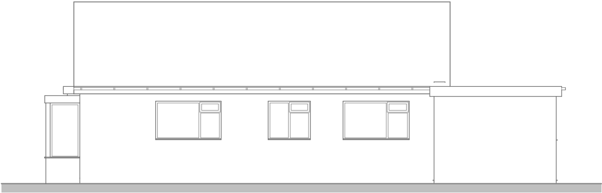
Side Elevation
