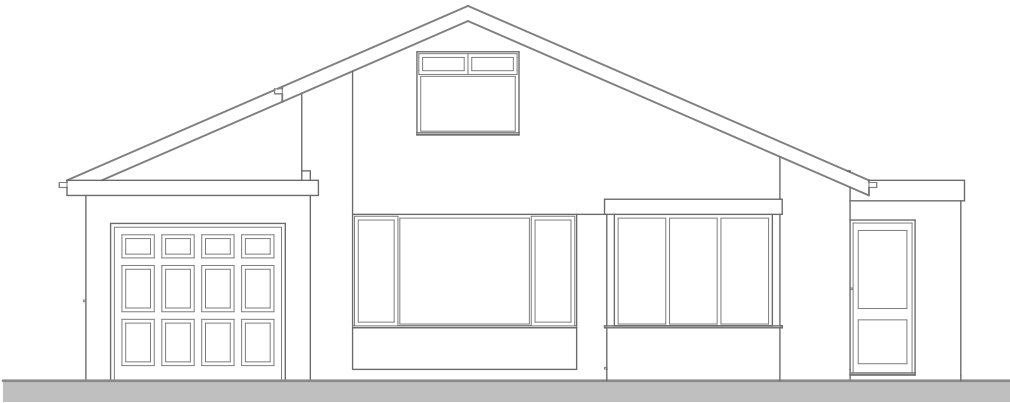
Front Elevation
