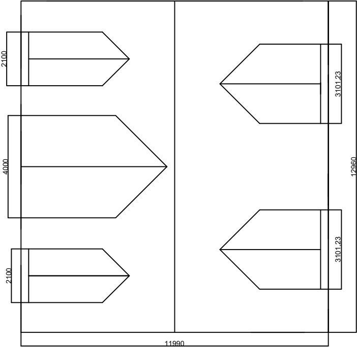
ROOF PLAN
