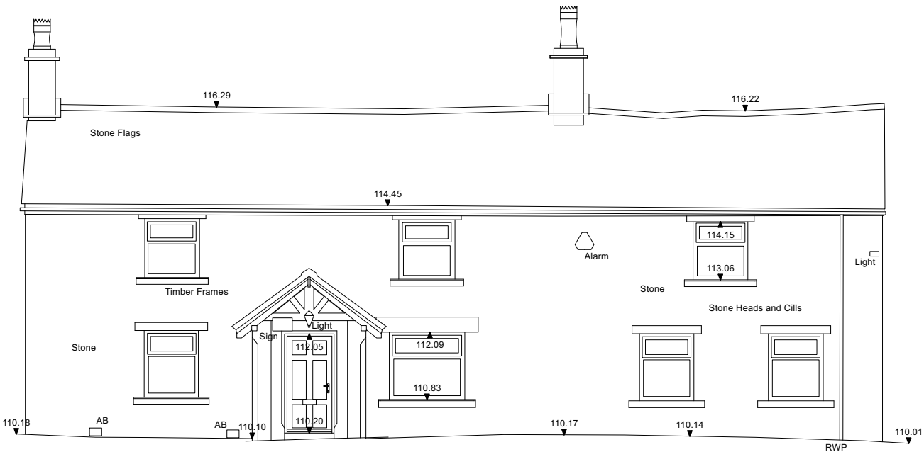
north elevation
