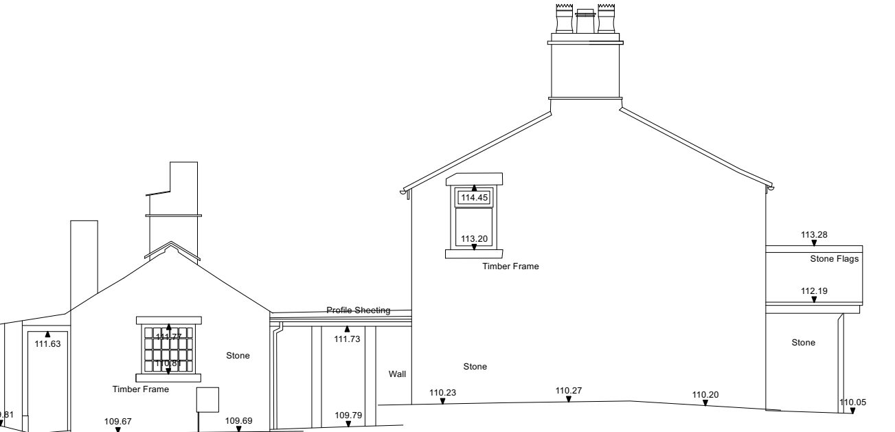
east elevation
