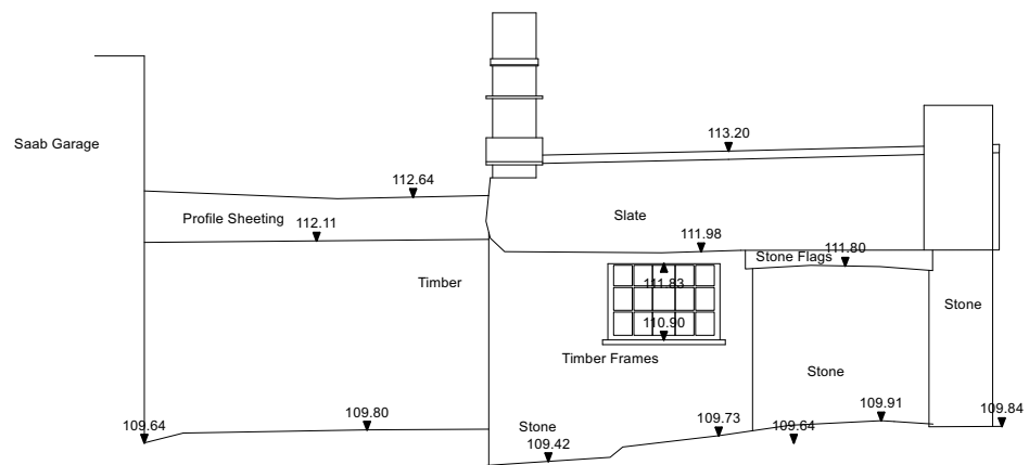
south elevation (outbuilding)
