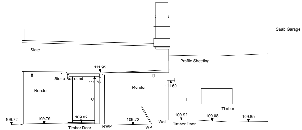
north elevation (outbuilding)
