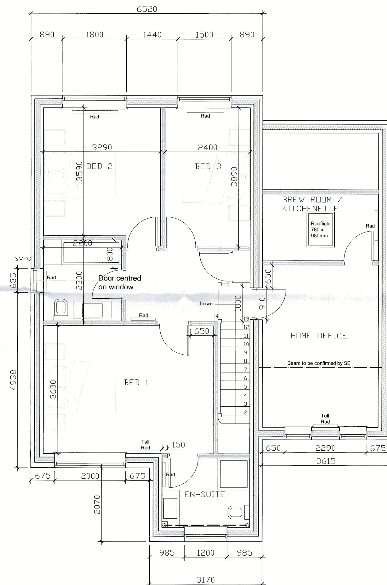
First Floor Plan 1:50 Scale
