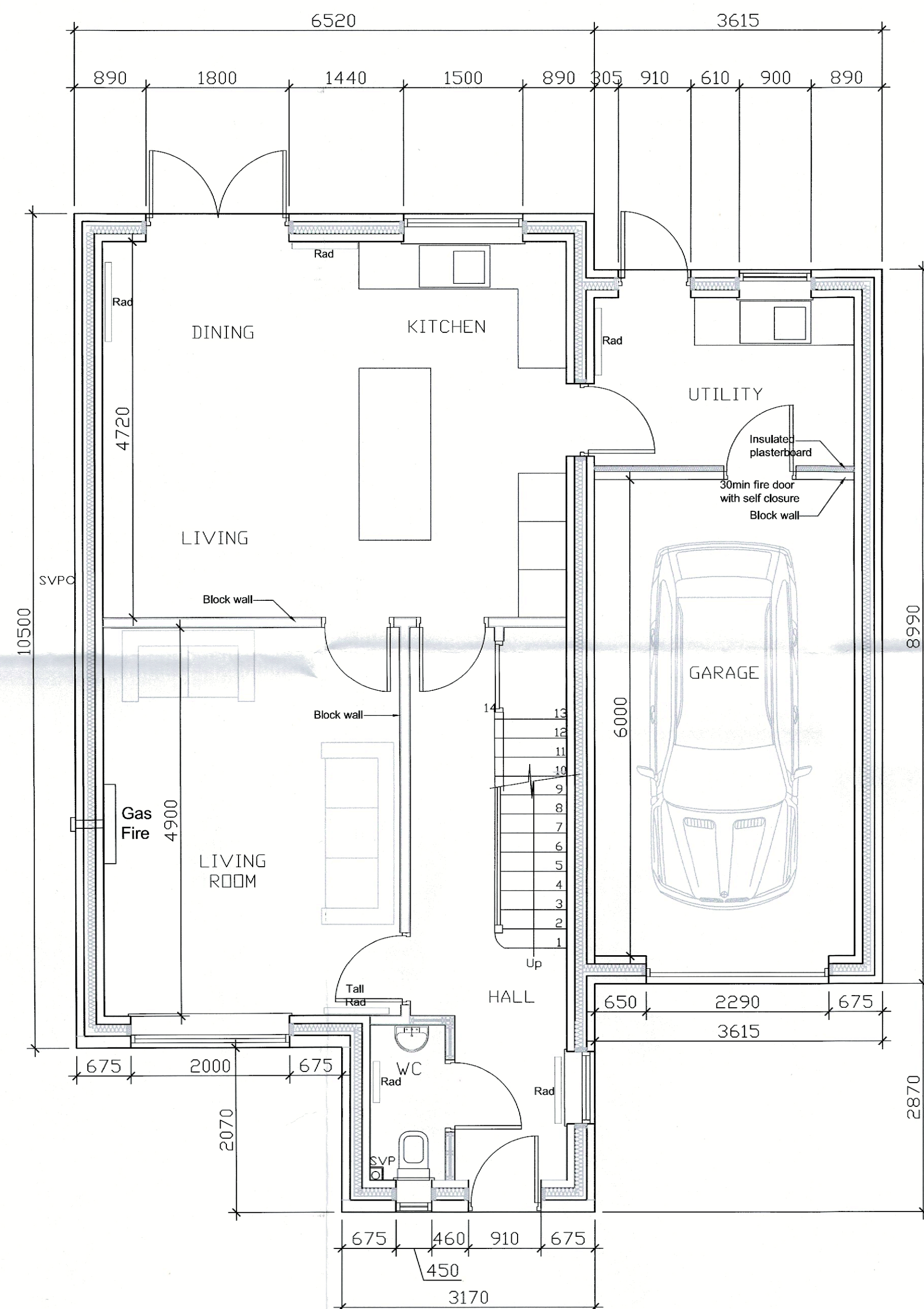
Ground Floor Plan 1:50 Scale
