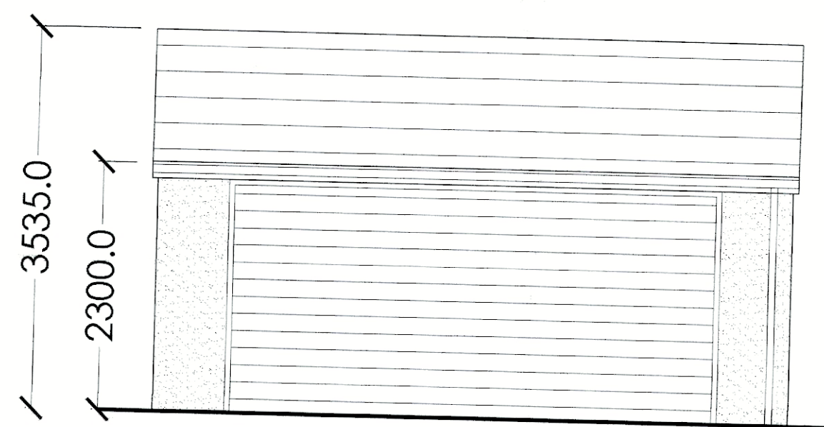
EAST ELEVATION
