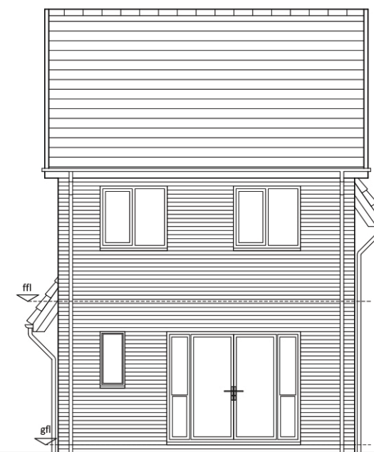
Rear Elevation
