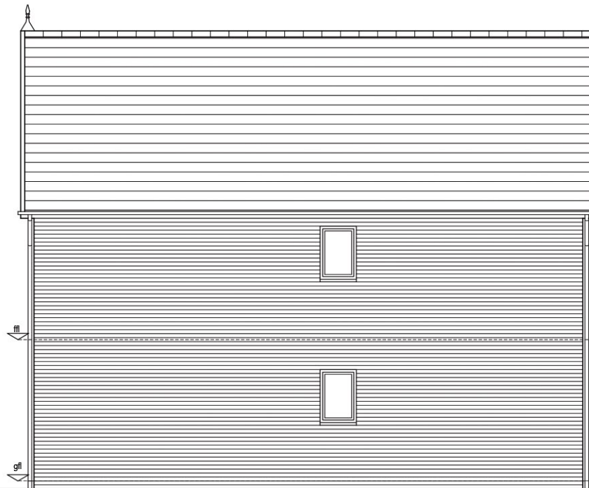
Side Elevation - Right / Left
