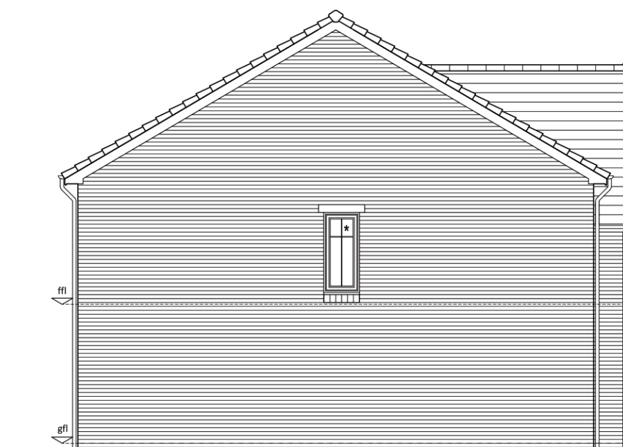
Side Elevation - Left
