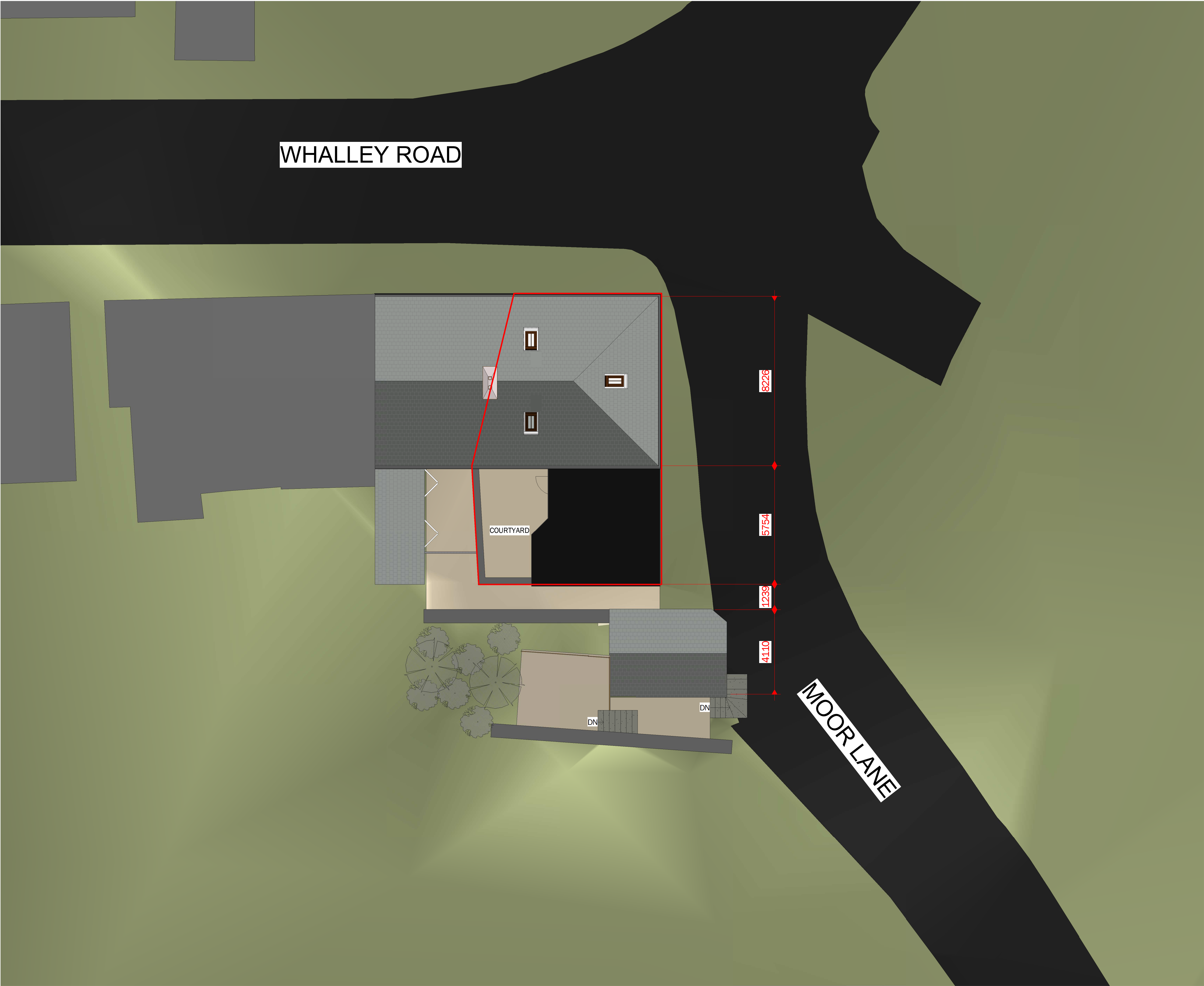
1 PROPOSED SITE PLAN 1 : 100
