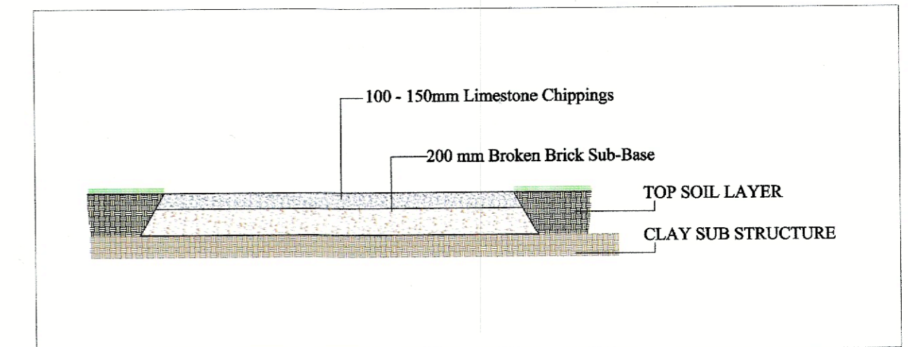
TRACK CROSS - SECTION Scale = 1:50
