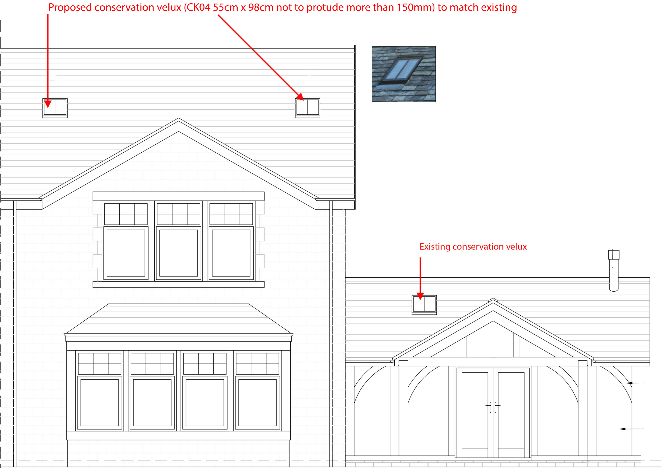
West Elevation
