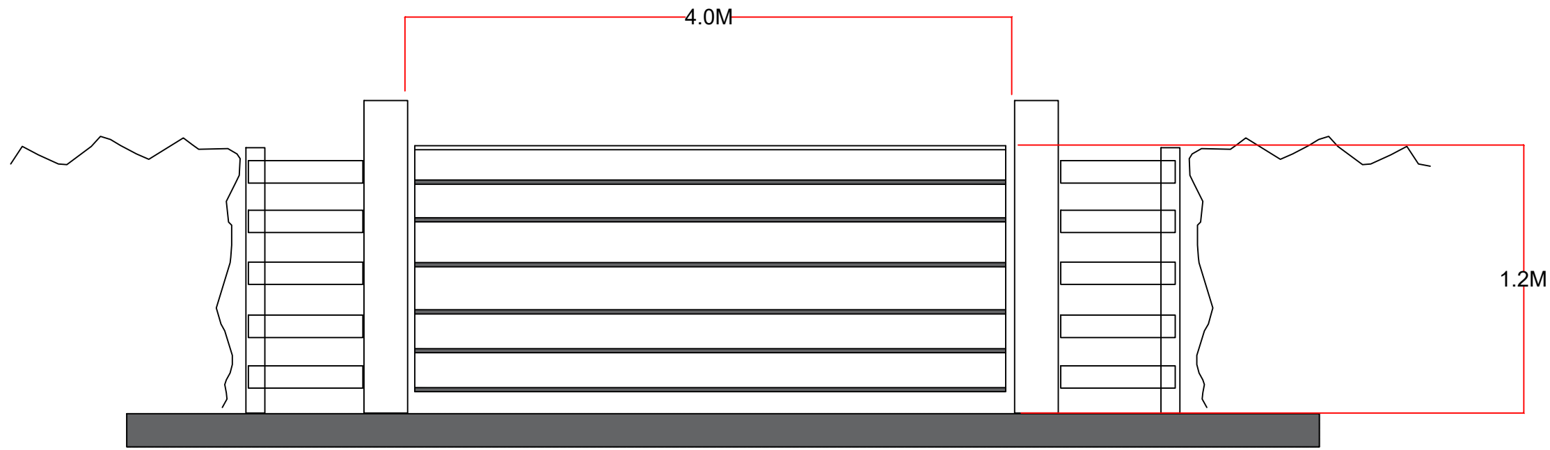
ELEVATION OF THE NEW GATE ENTRANCE
