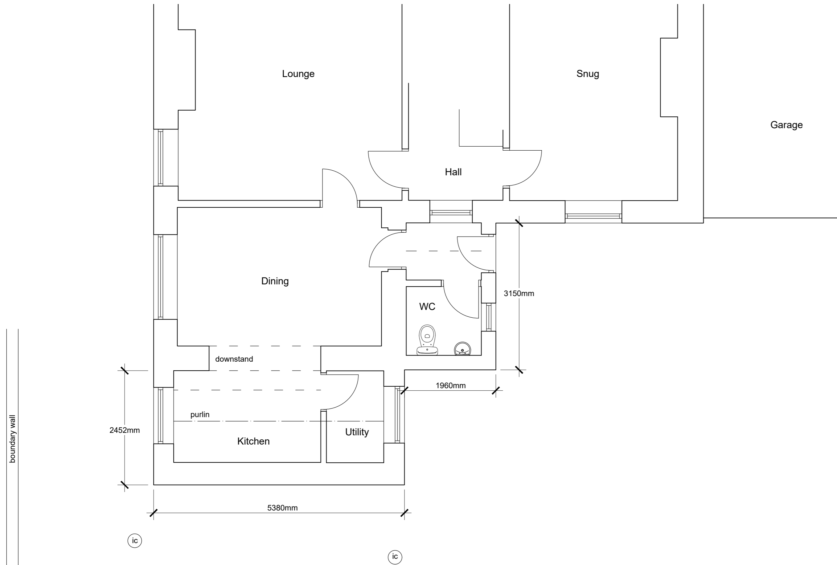
Part Ground Floor Plan 1:50
