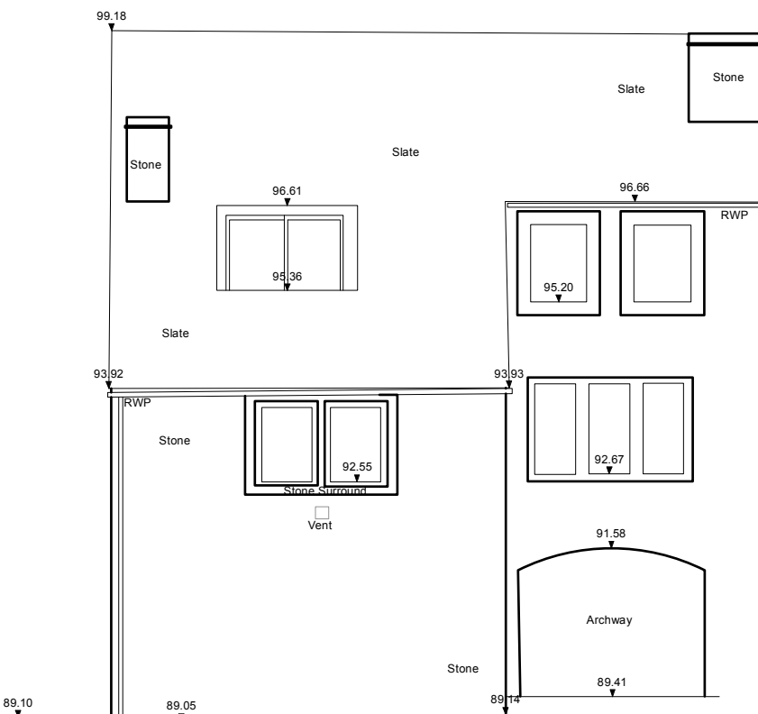
West Elevation
