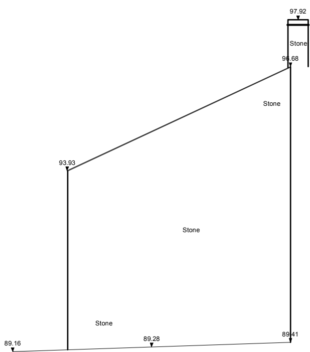
South Elevation
