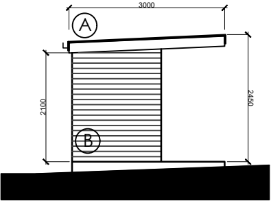
East Elevation
