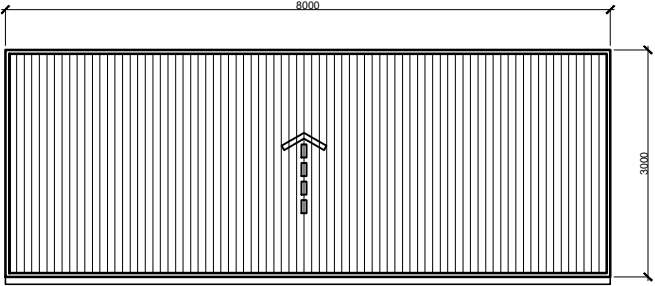
Roof Plan
