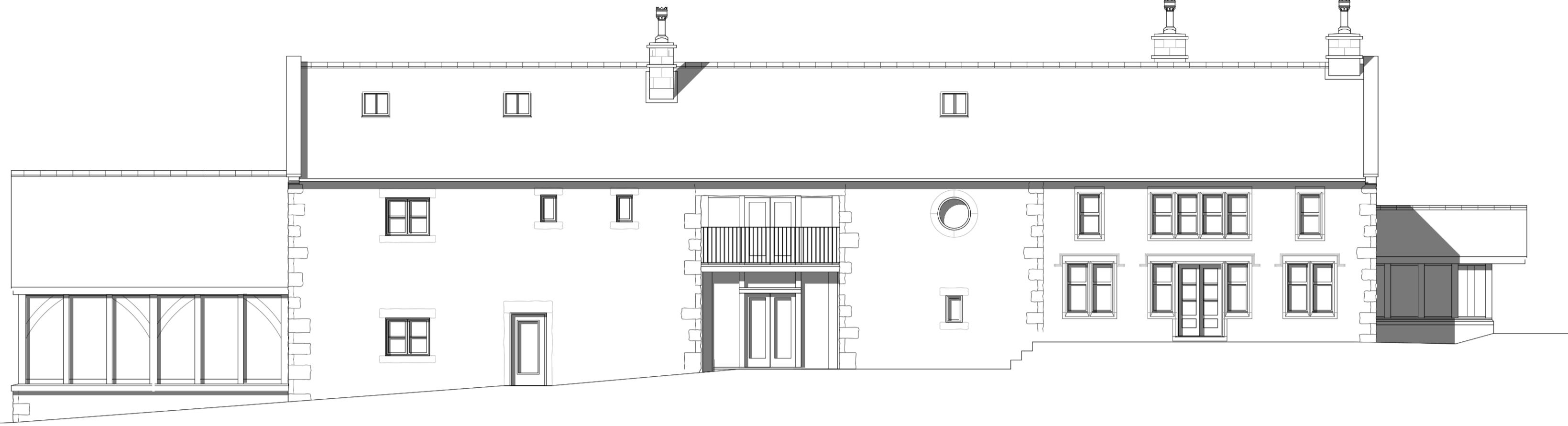
Existing Elevation A (South, Rear) SCALE 1:100
