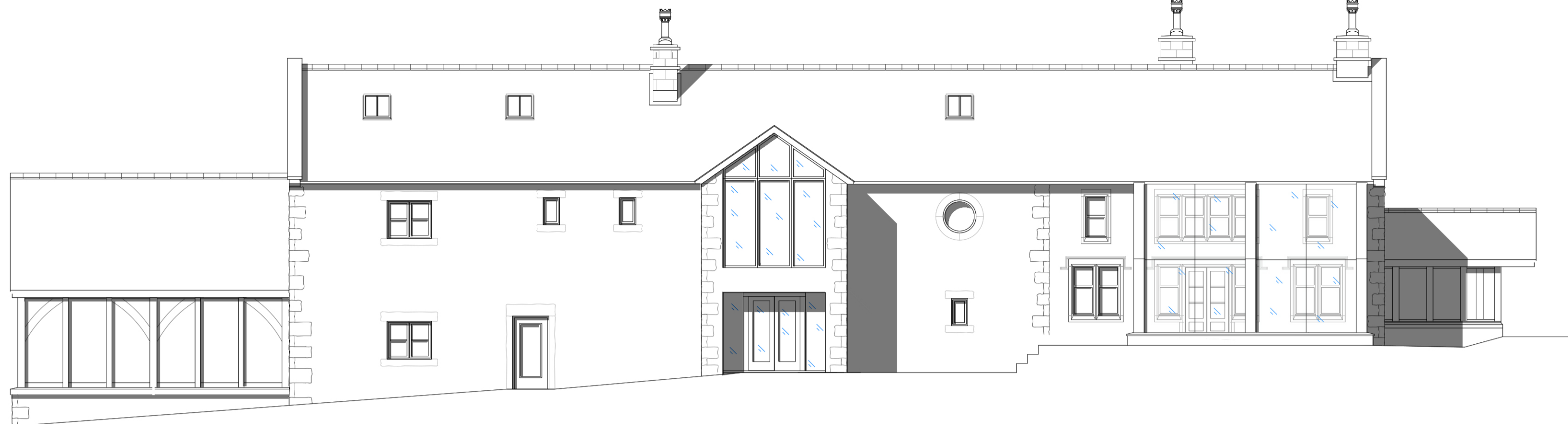
Proposed Elevation A (South, Rear) SCALE 1:100
