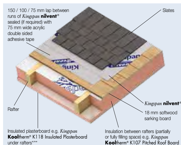
Figure 1d – Insulation Between Rafters – Sarking Board & Natural Slates
