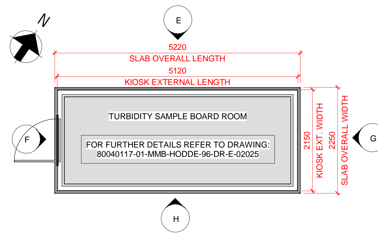
TURBIDITY SAMPLE BOARD ROOM 1 : 50
