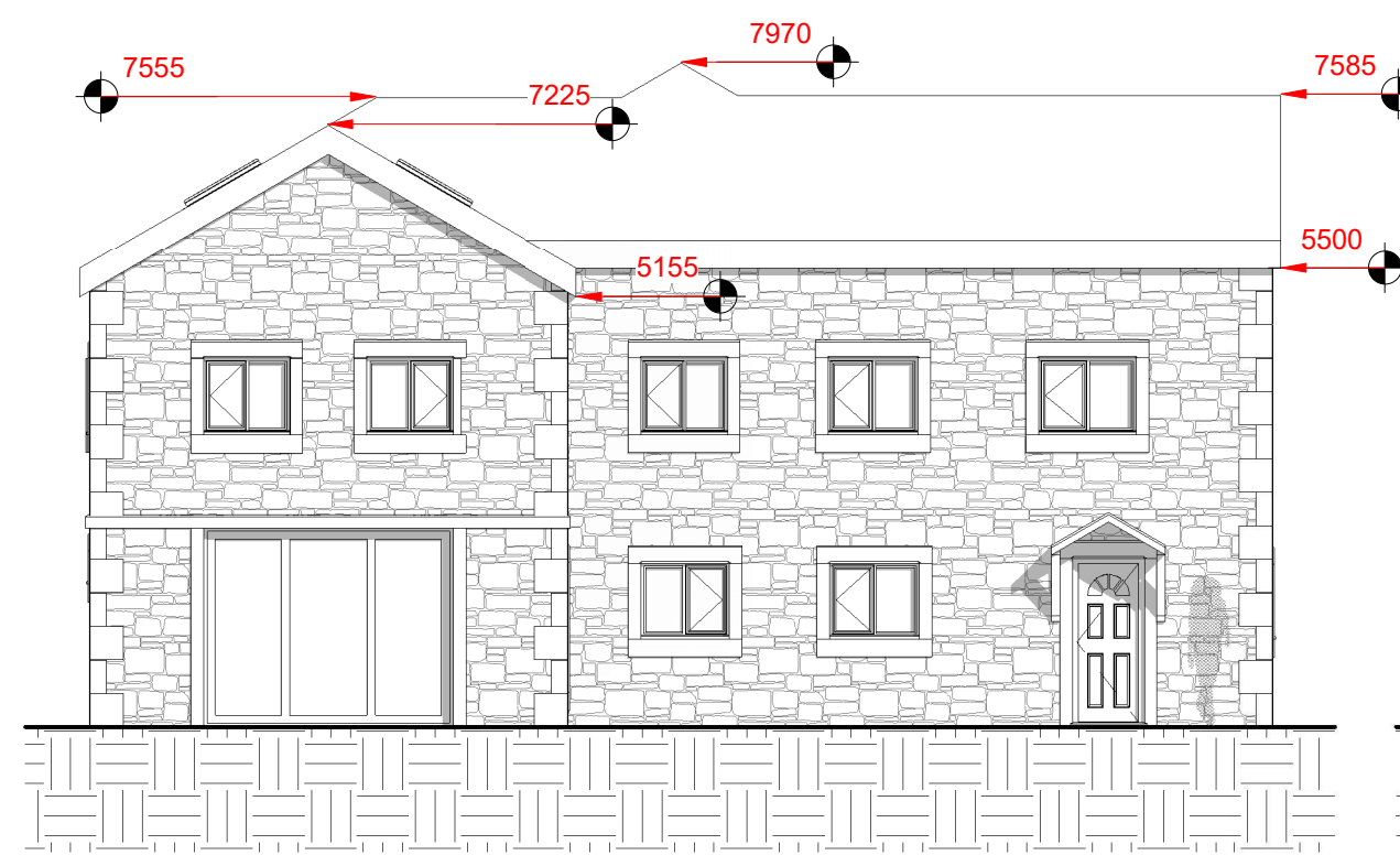
3 PROPOSED NORTH 1 : 100
