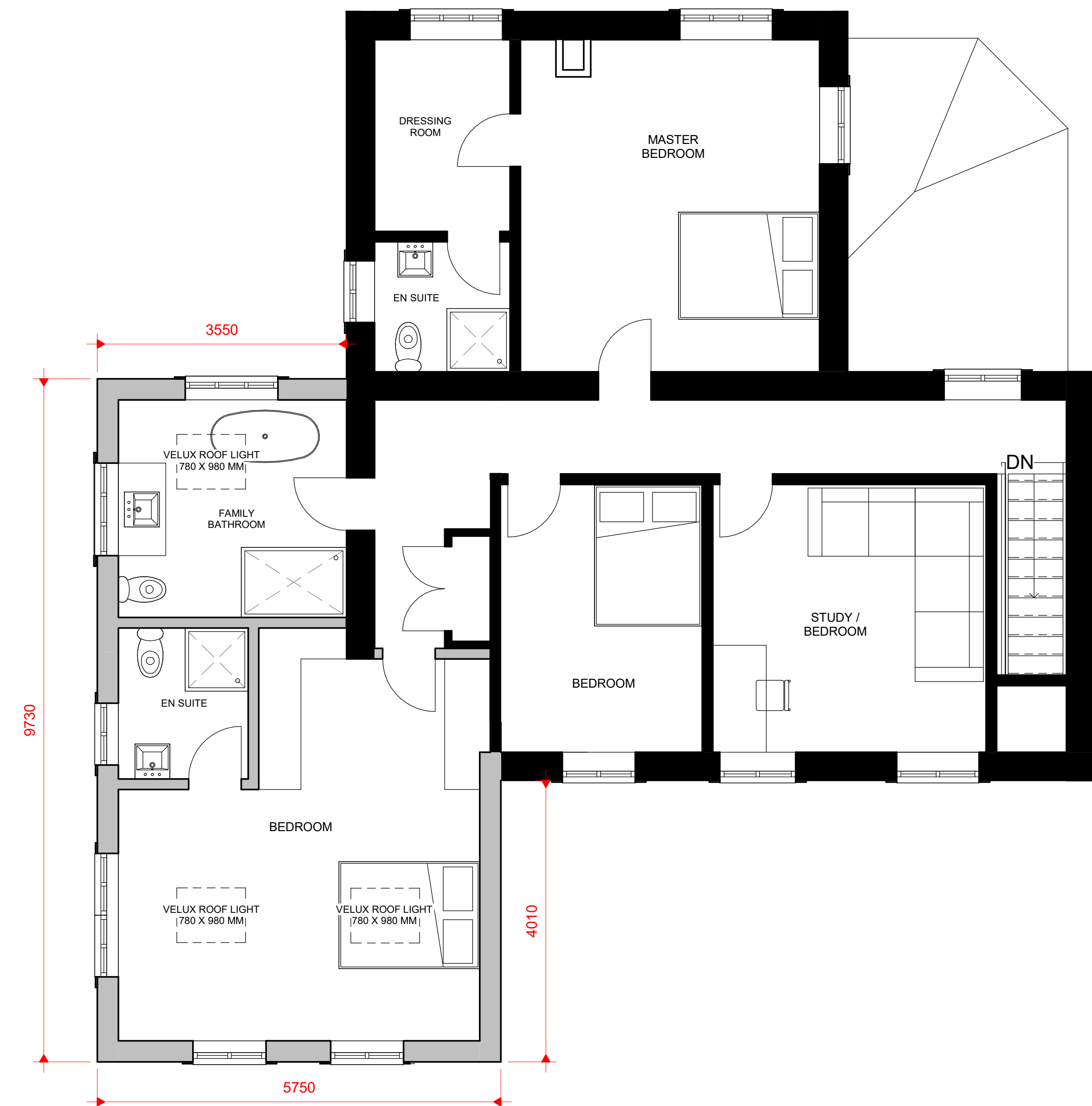
2 1 PROPOSED FIRST FLOOR 1 : 50
