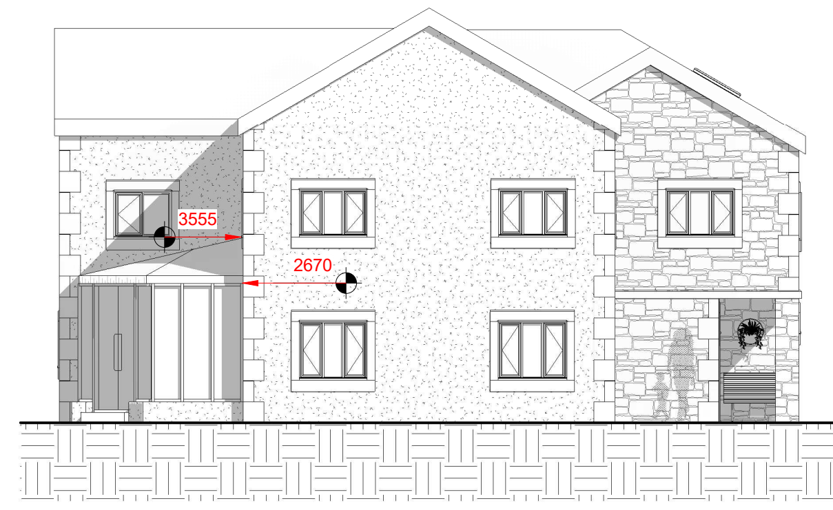
5 PROPOSED SOUTH 1 : 100
