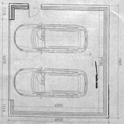
Proposed Ground Floor Plan 1:50 Scale
