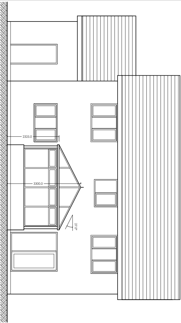
REAR ELEVATION AS EXISTING 1.100 @ A3
