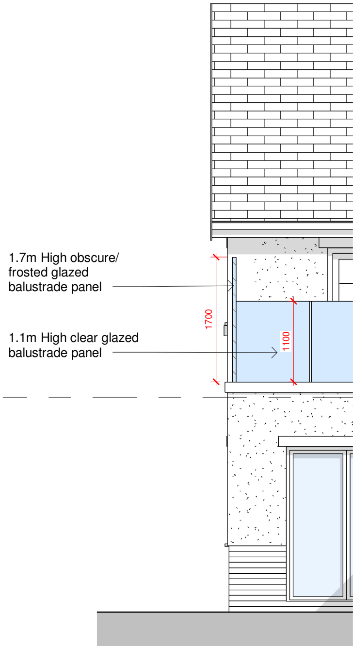
Typical Proposed Balustrade Front Elevation 1 : 50
