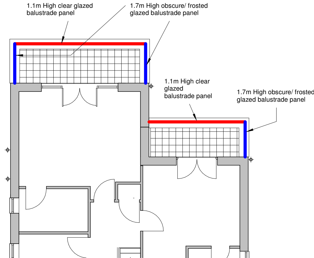
01_Proposed Balcony Plan 1 : 100
