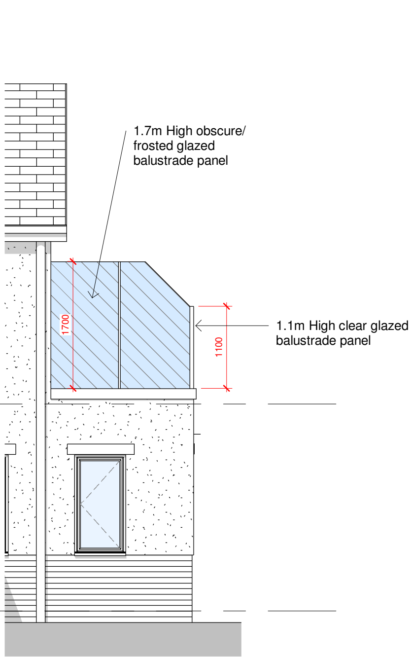
Typical Proposed Balustrade Side Elevation 1 : 50
