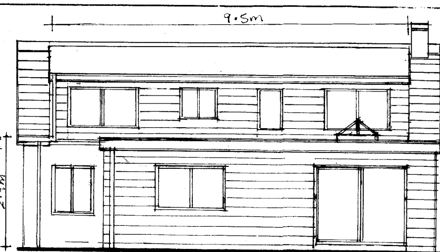
WEST ELEVATION
