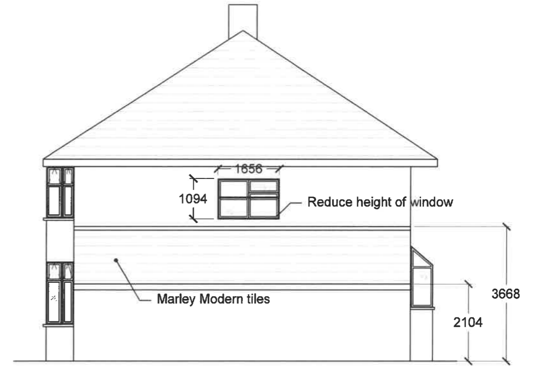
SIDE ELEVATION
