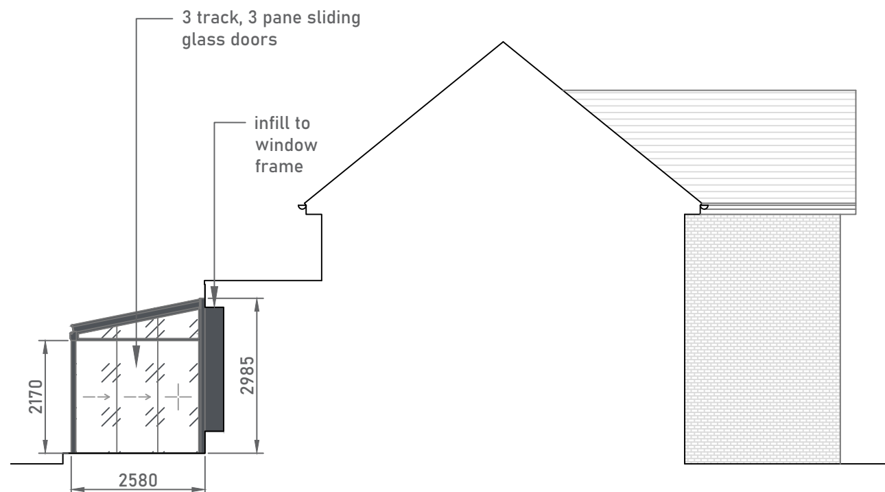
SIDE SECTION
