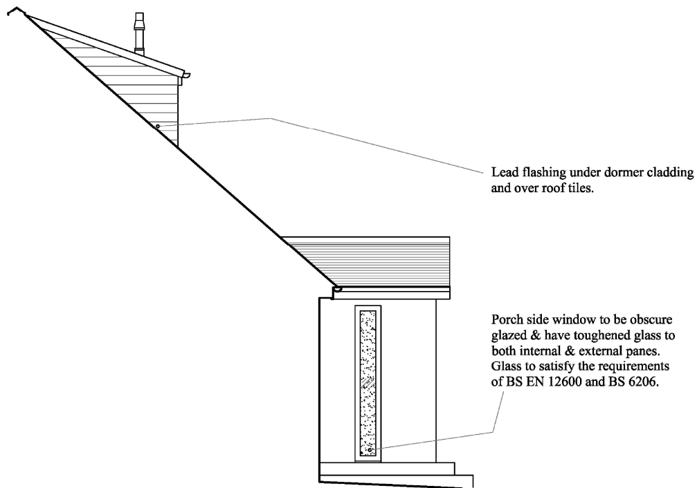
SIDE (NORTH EAST FACING) ELEVATION Proposed
