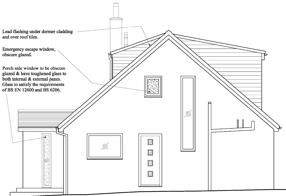
SIDE (SOUTH WEST FACING) ELEVATION Proposed
