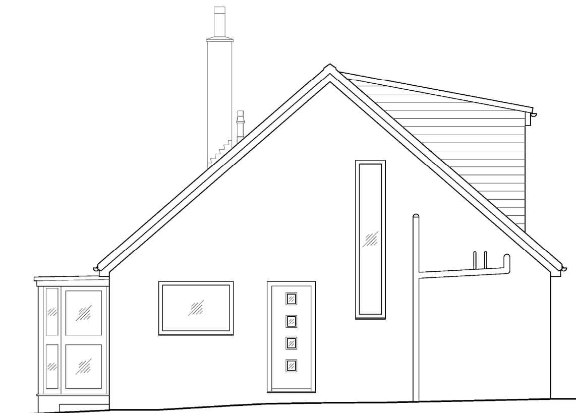
SIDE (SOUTH WEST FACING) ELEVATION Existing
