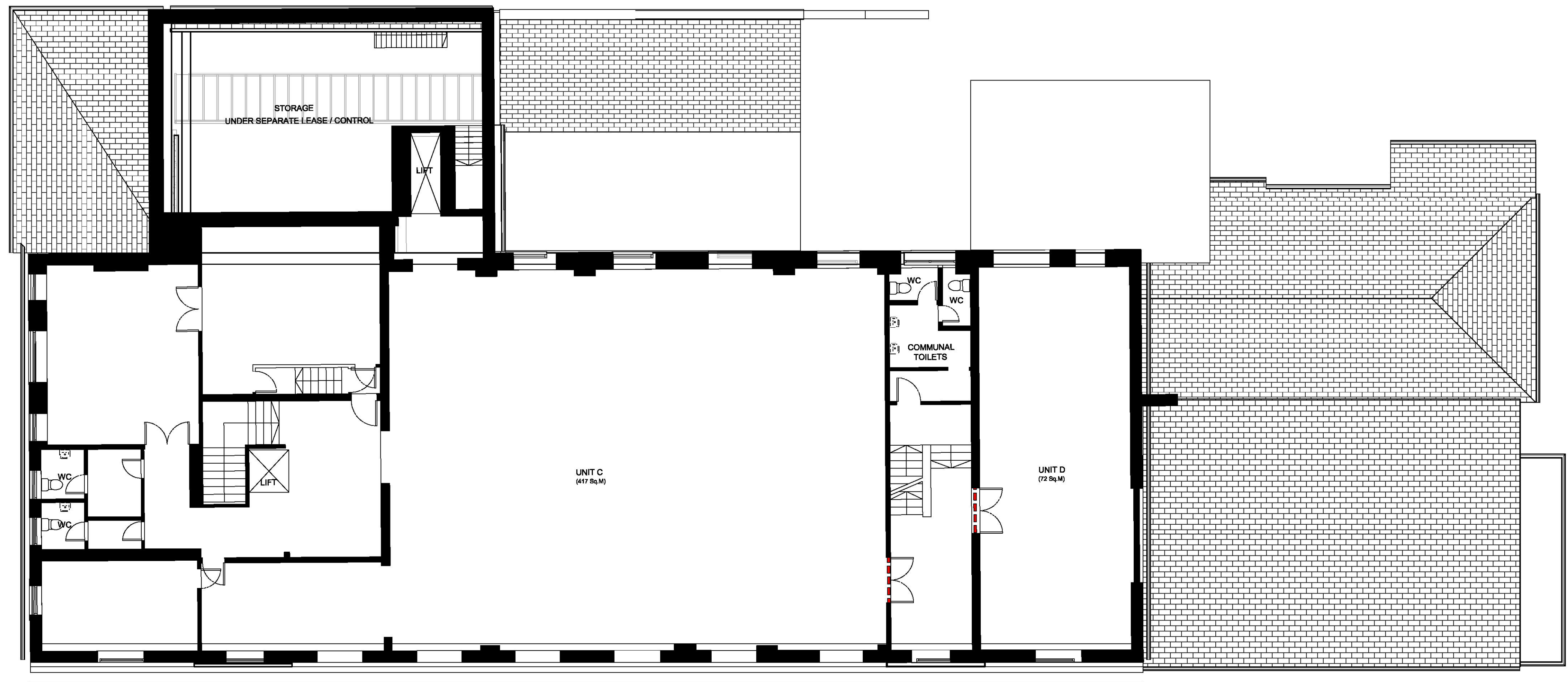
2 Existing First Floor 1 : 100
