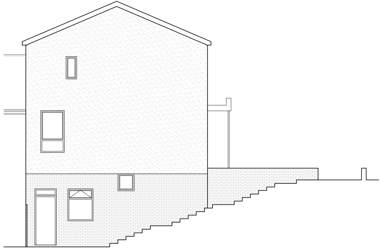
EXISTING SIDE ELEVATION 1:100 @ A3
