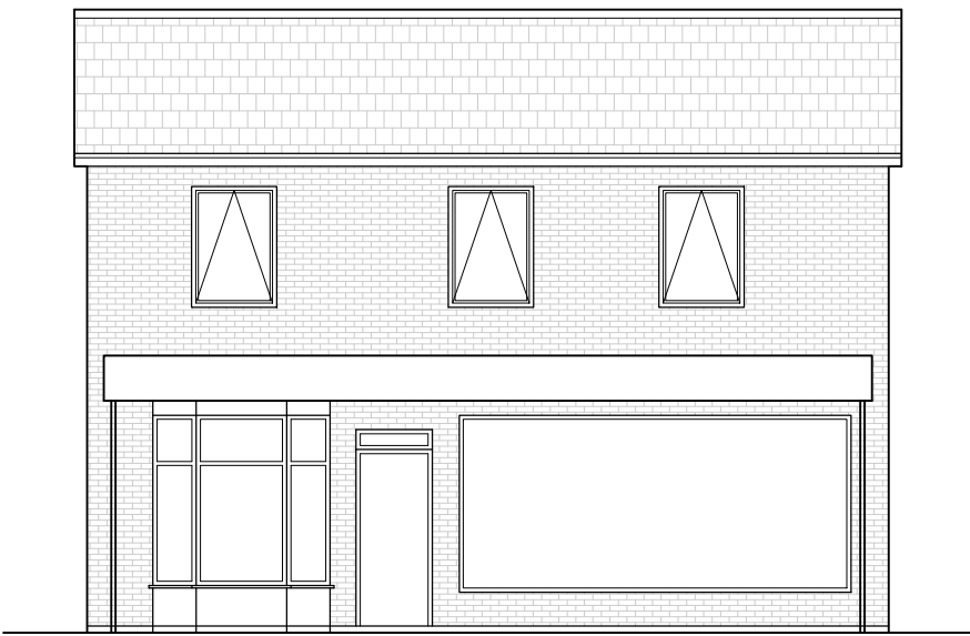
EXISTING FRONT ELEVATION 1:100 @ A3
