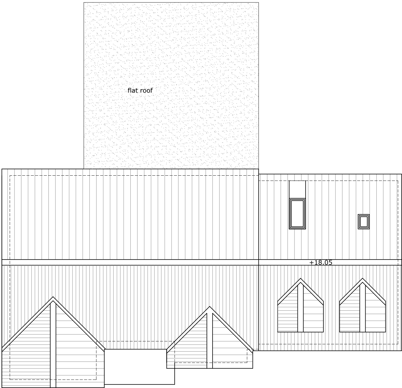
ROOF PLAN
