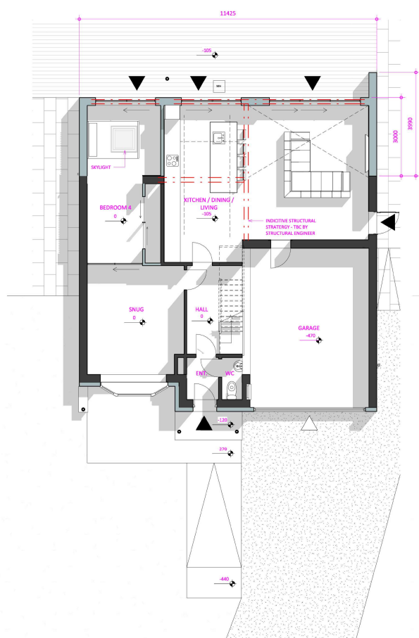
1 PROPOSED GROUND FLOOR 1 : 50
