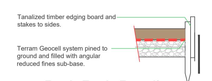
Porous Bark Path Detail Scale@1:10
