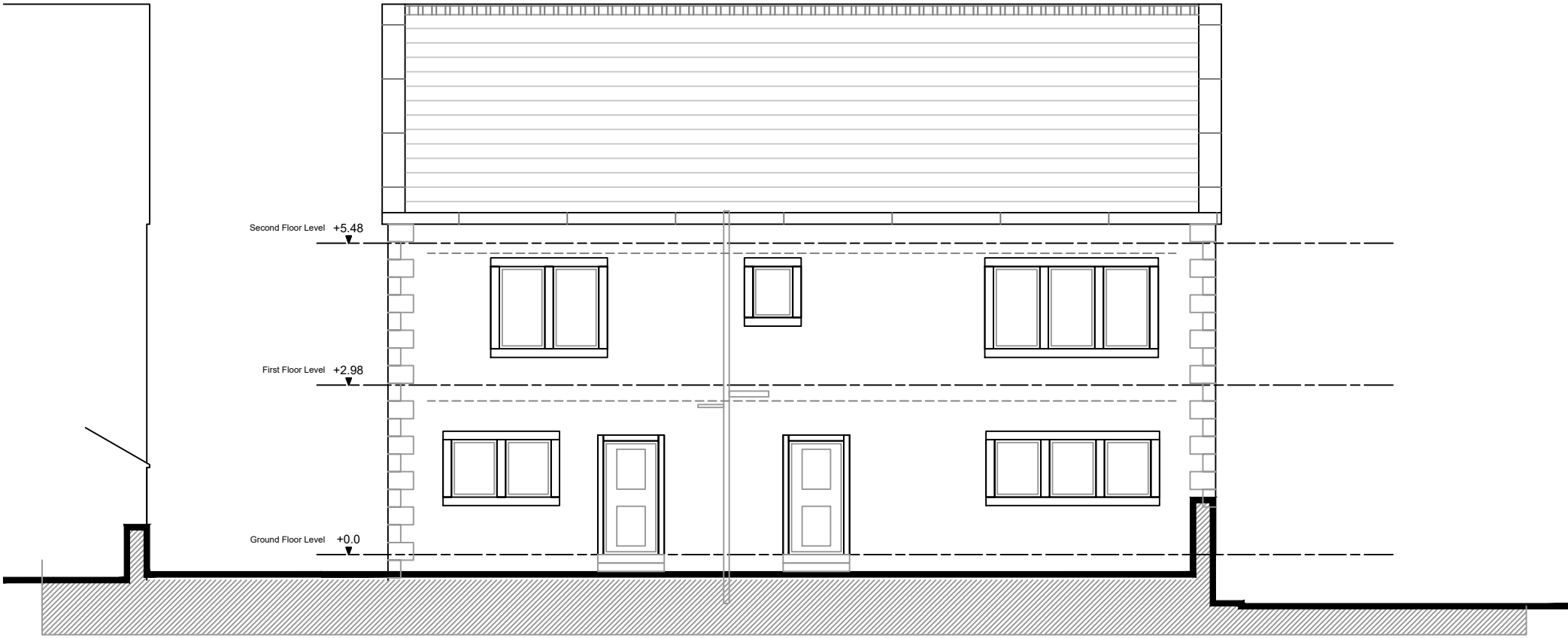
3 Existing Rear Elevation Scale 1:100
