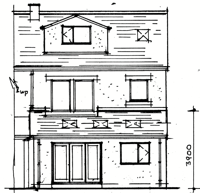
proposed elevations
