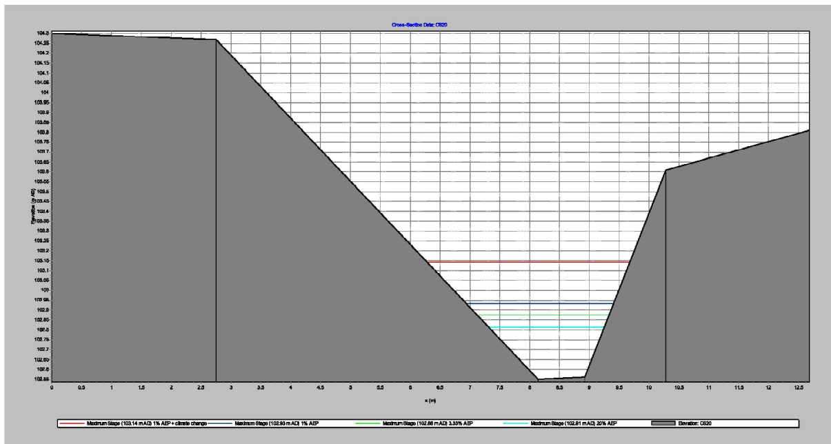
Figure F.18 Peak levels at cross section CS20
