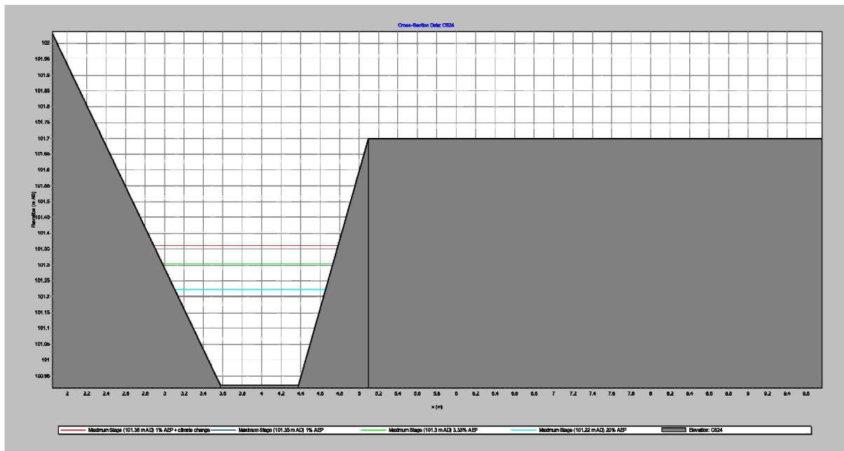
Figure F.22 Peak levels at cross section CS24
