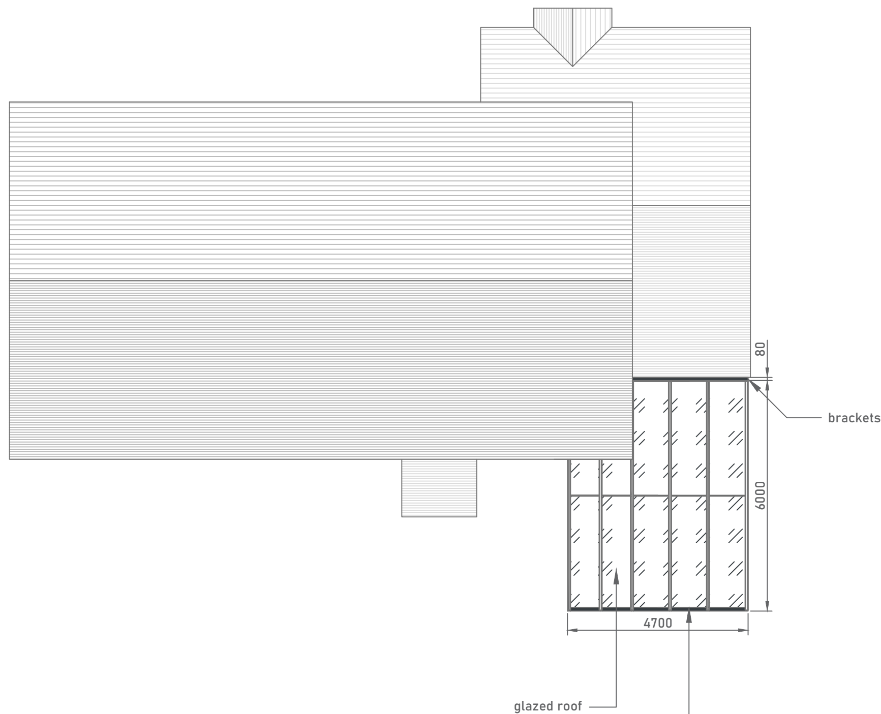
ROOF PLAN
