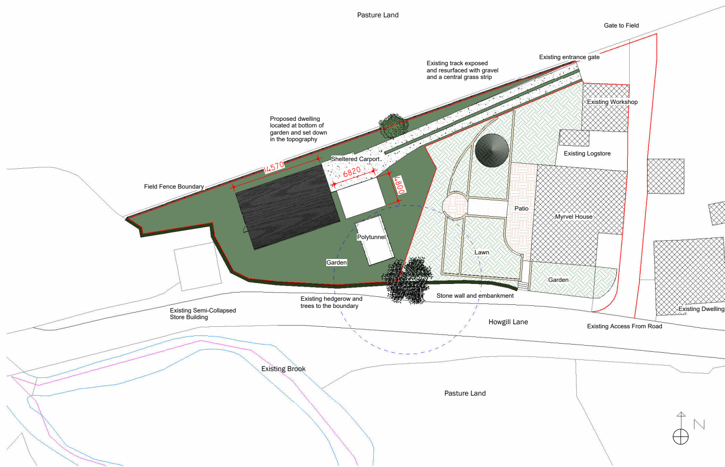
1 PROPOSED SITE PLAN 1 : 200
