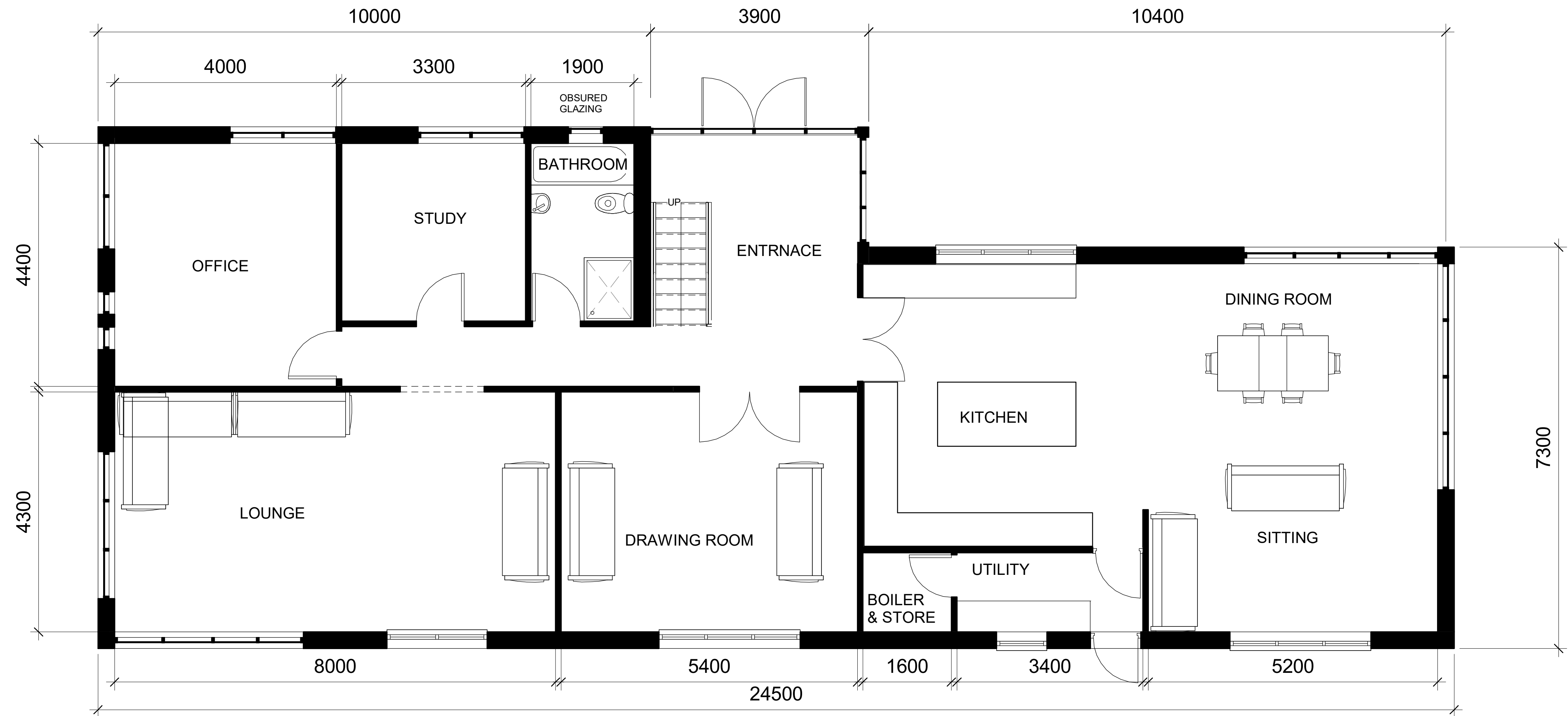
1 0 GROUND FLOOR 1 : 50
