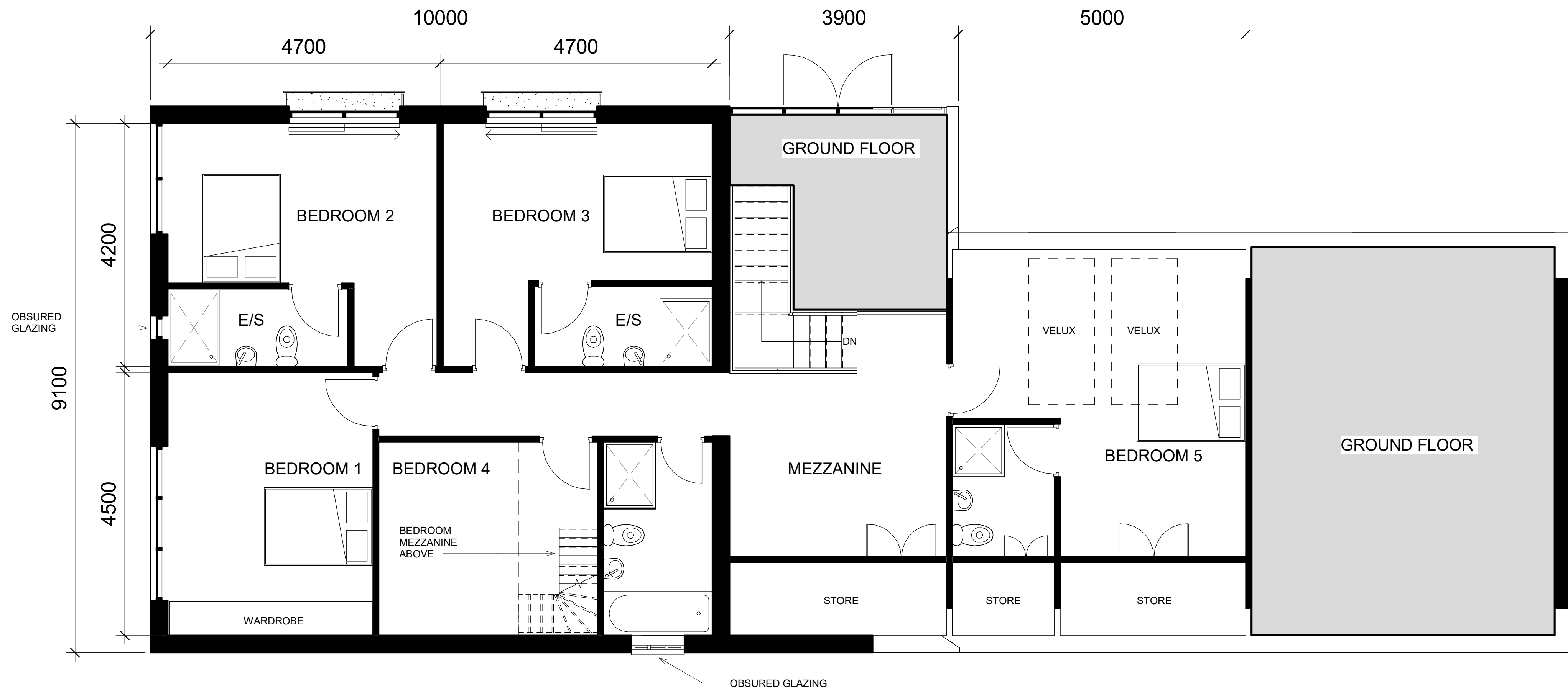
2 1 FIRST FLOOR 1 : 50
