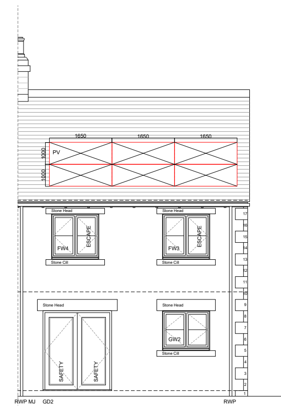
Rear Elevation (North)
