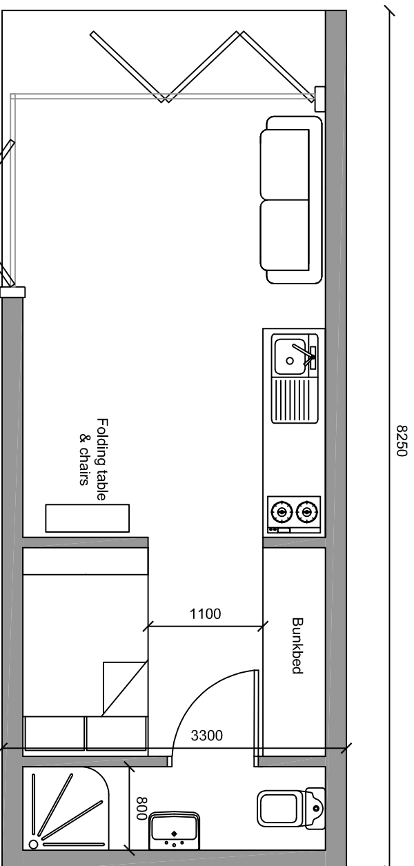
FLOOR PLAN
