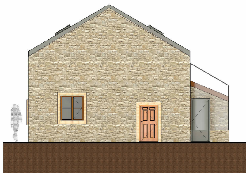
3 PROPOSED NORTH ELEVATION 1 : 50
