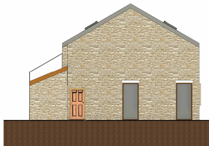
1 PROPOSED SOUTH ELEVATION 1 : 50
