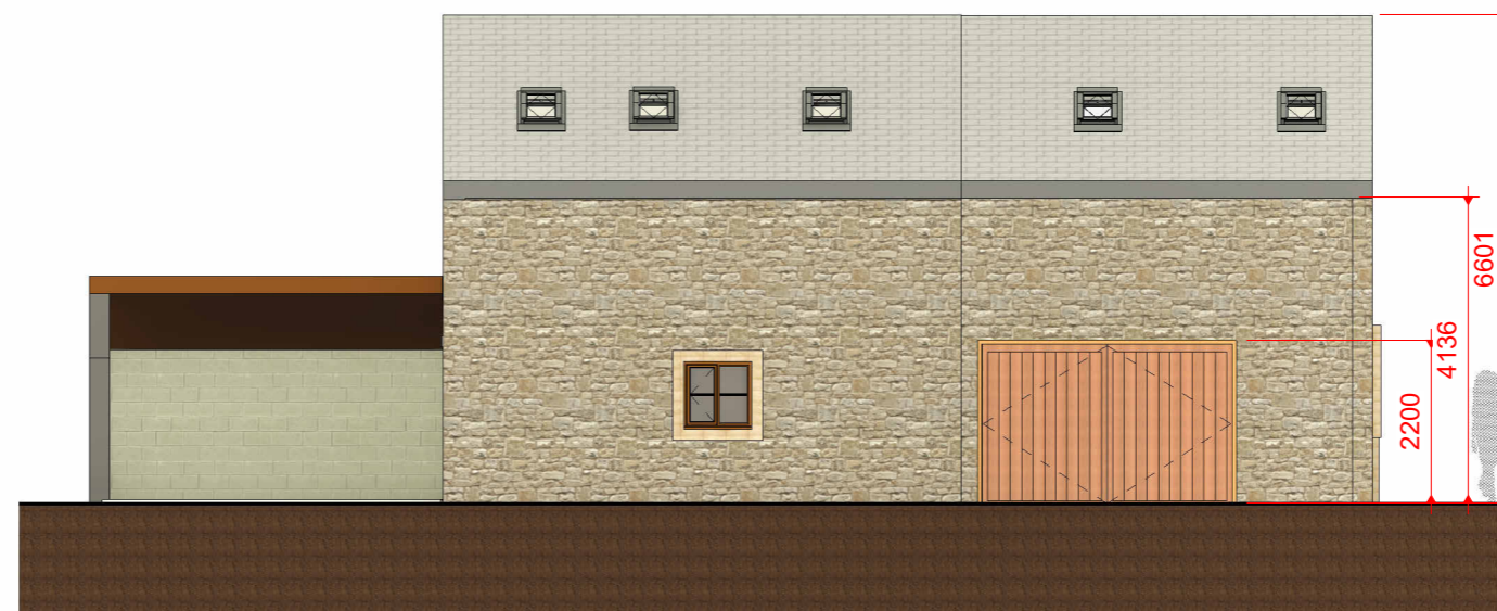
2 PROPOSED EAST ELEVATION 1 : 50
